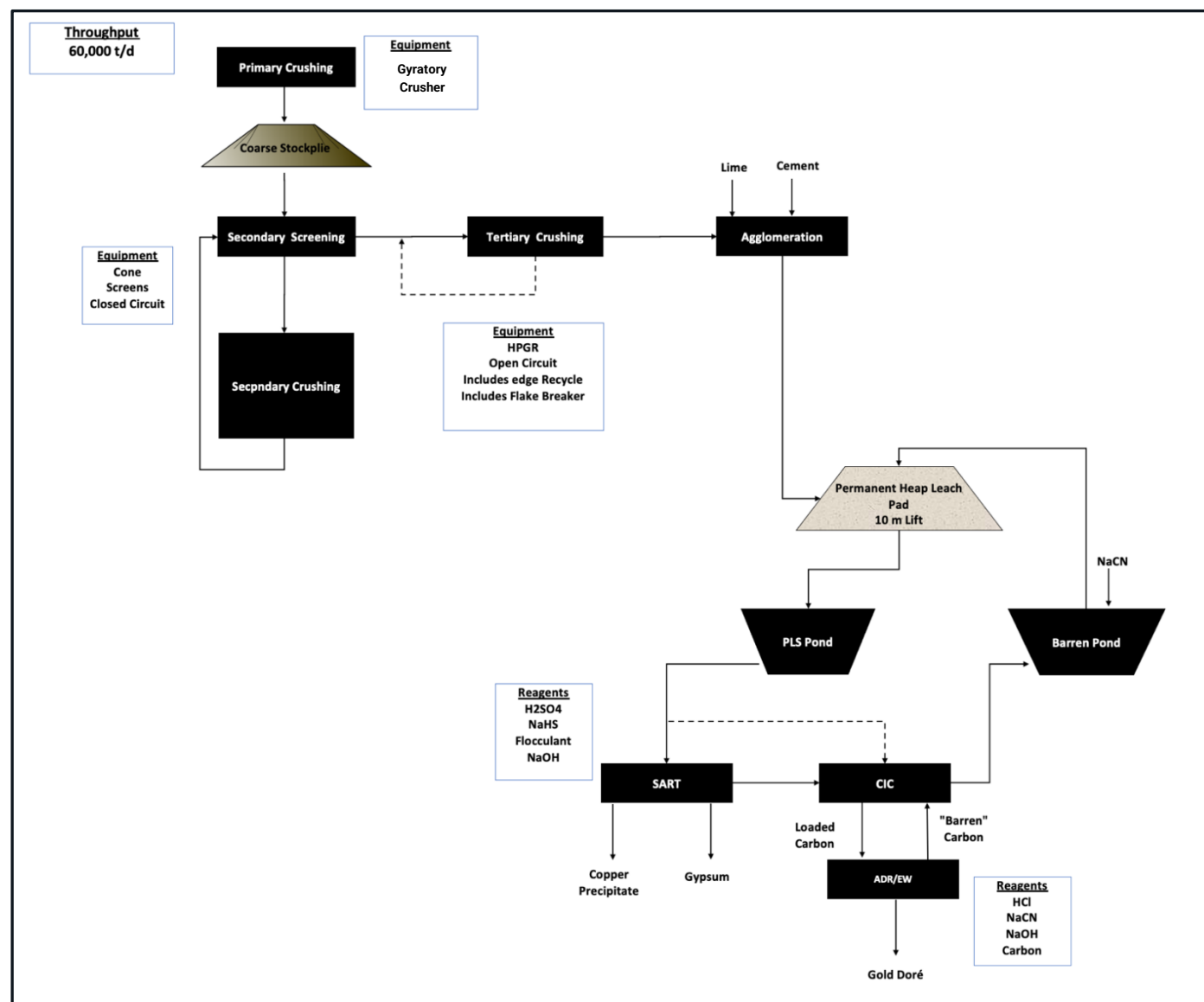
Figure 17-1: Process Flowsheet
