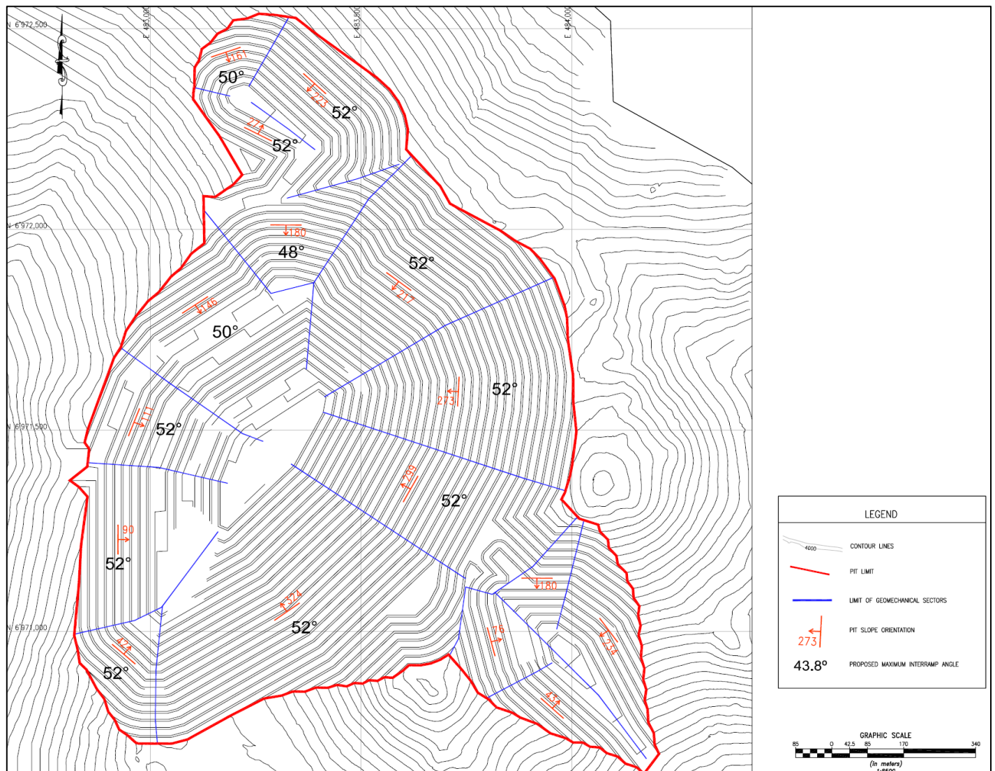
Figure 16-2: Geotechnical Sectors
