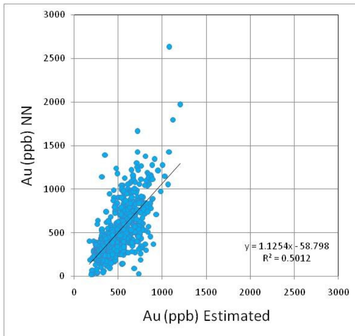
Figure 14-34: Dispersion Graph for DO (Norte 110/111), All Samples
