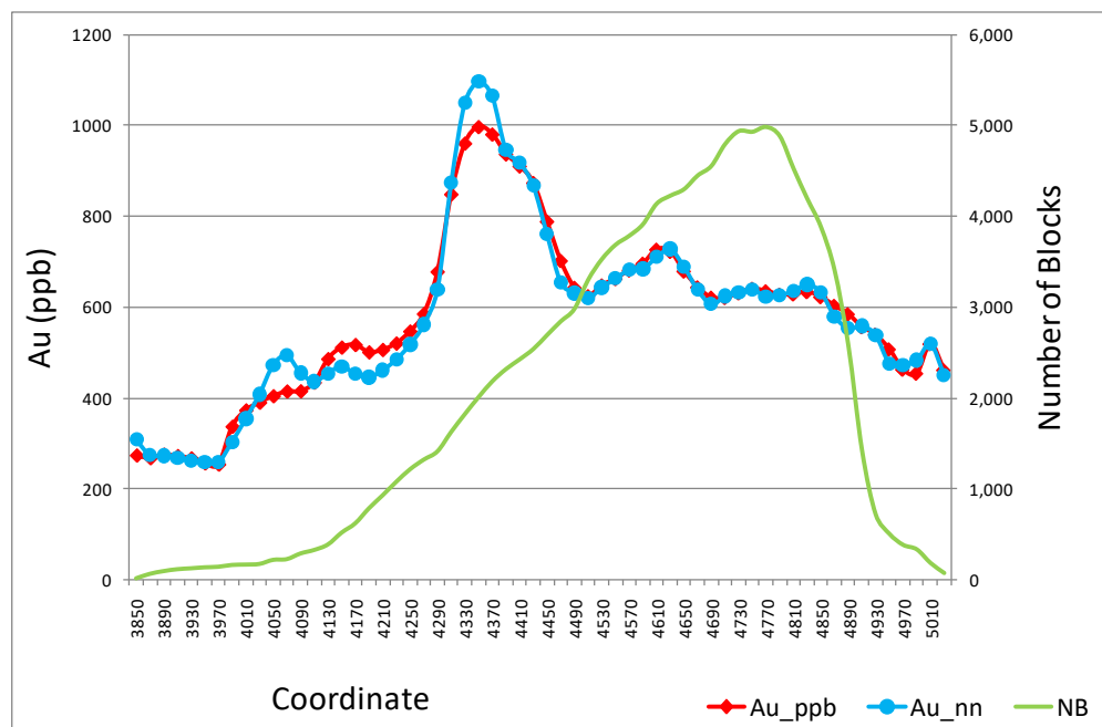
Figure 14-32: Drift Analysis for the DO (Sur) Domain (Code 121) (Bench data are presented on the y-axis while cross-sectional data are presented on the x-axis)
