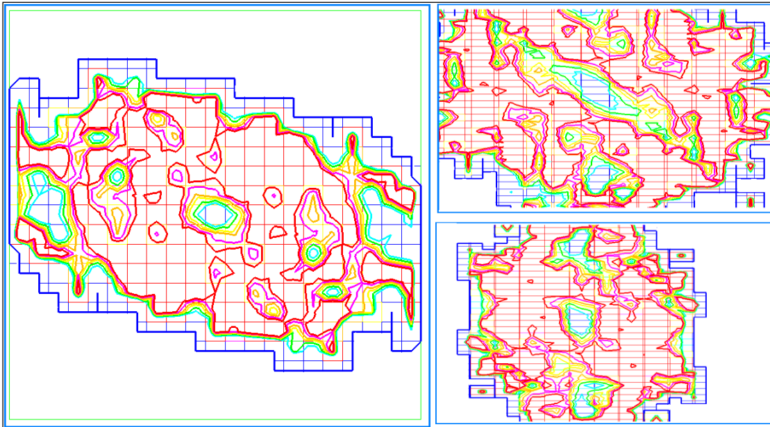
Figure 14-21: Variographic Map for the Veinlet Domain (Code 2002), DC Deposit
