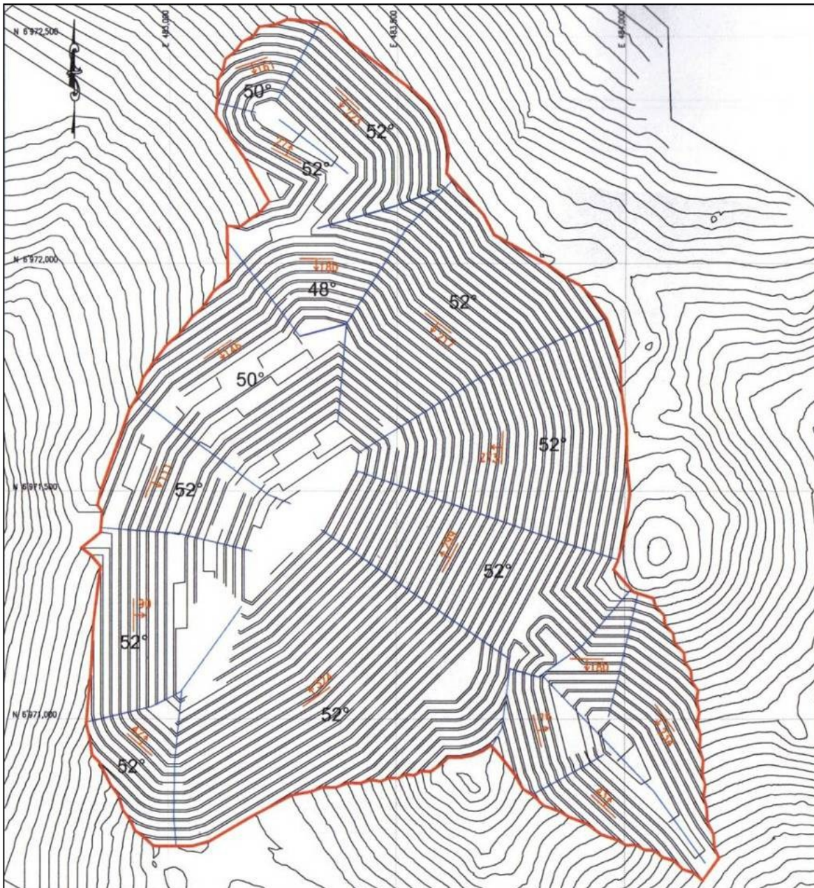
Figure 14-37: Preliminary Overall Wall Slope Sectors, Dorado Area Open Pits, Volcan Project
