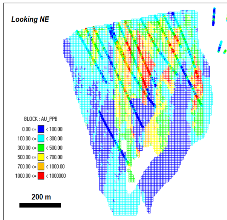
Figure 14-29: DO - Main Body – North End – Vertical Section
